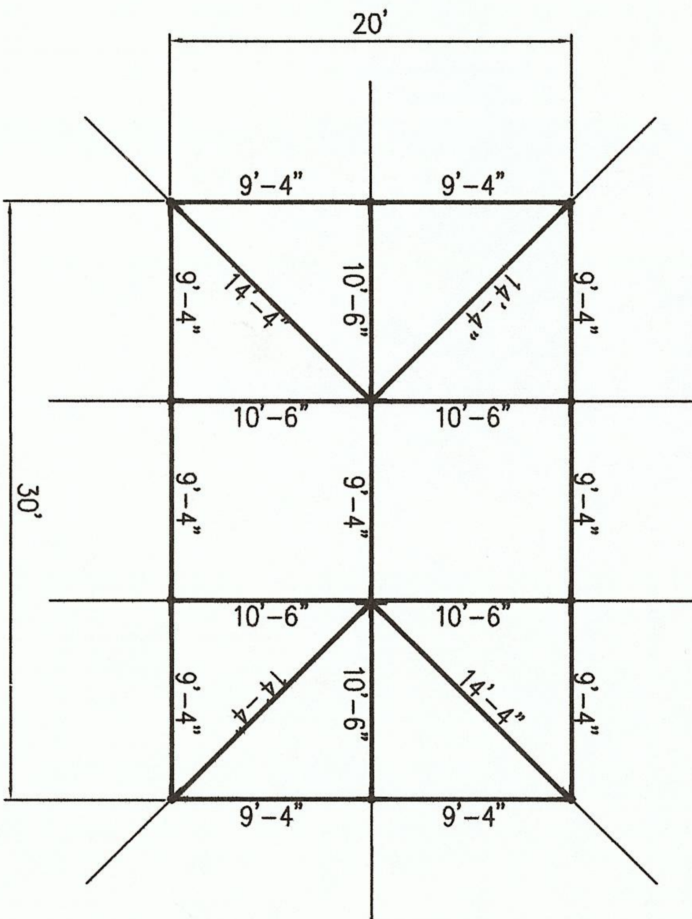
PLAN VIEW
