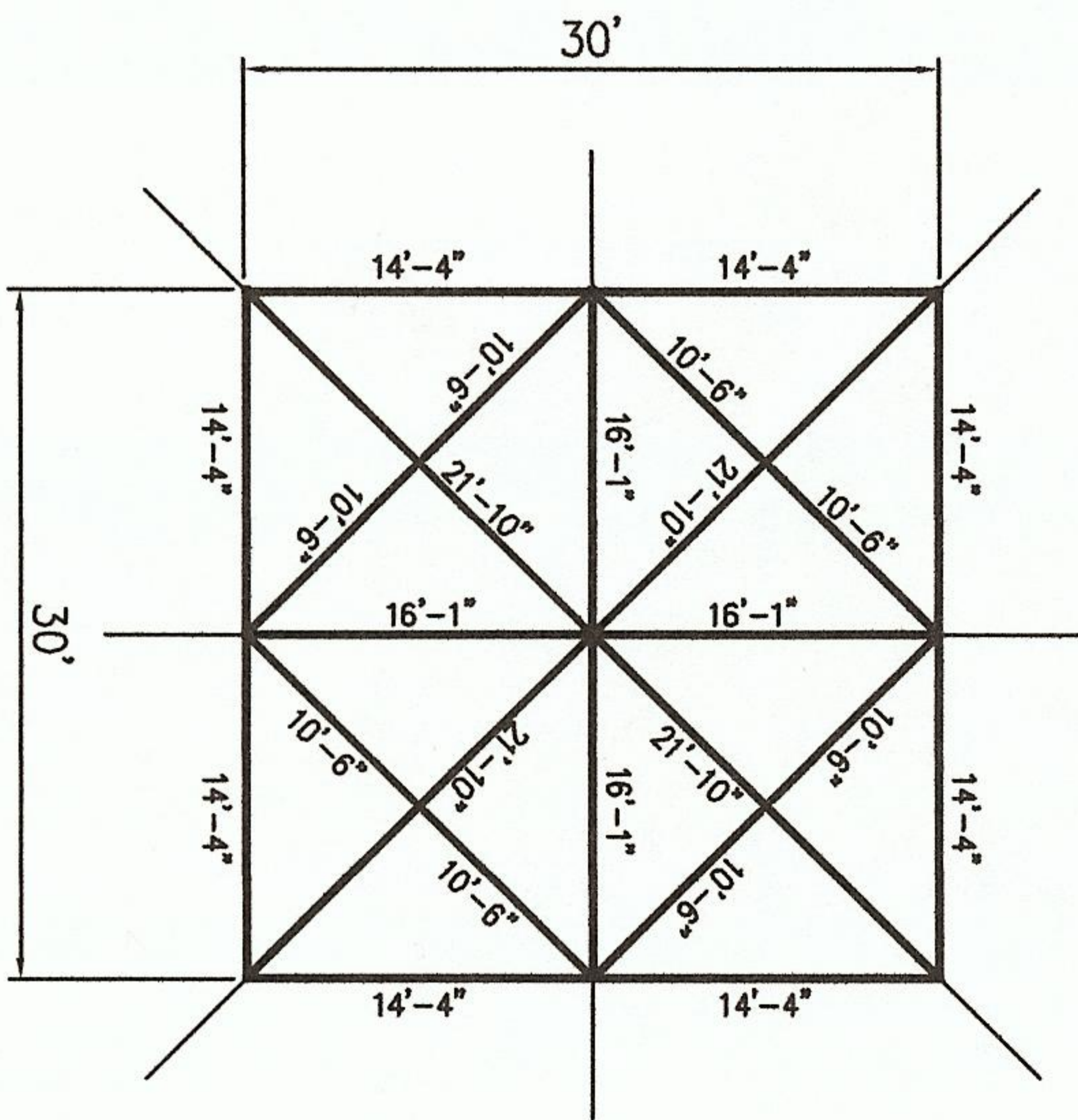
PLAN VIEW
