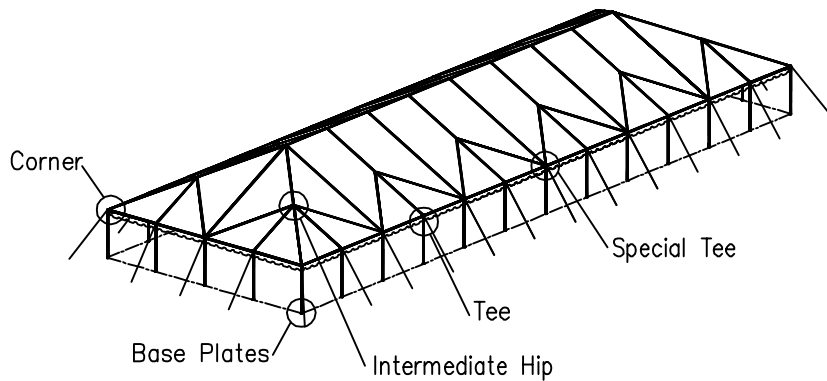
ISOMETRIC VIEW
