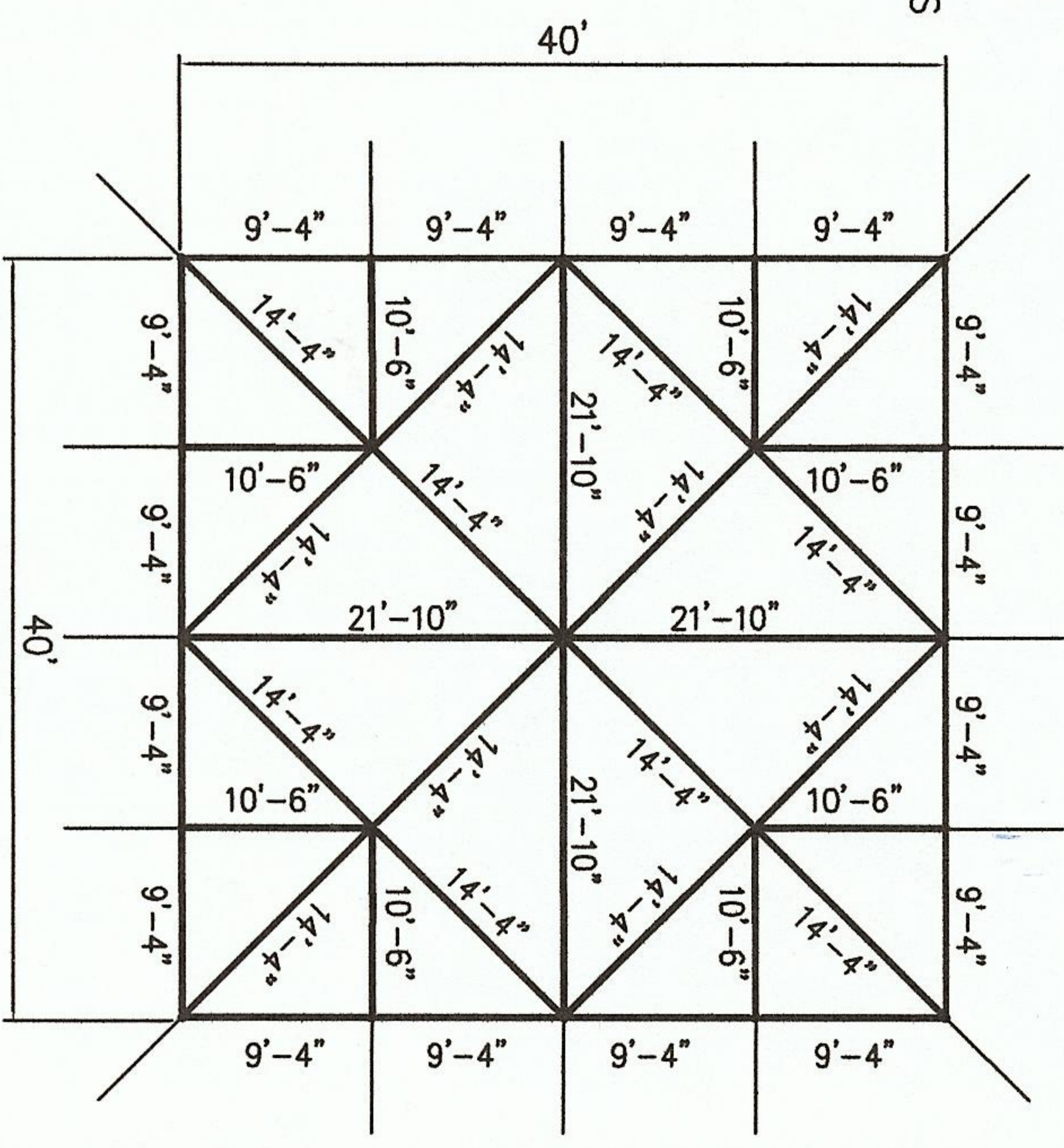
PLAN VIEW
