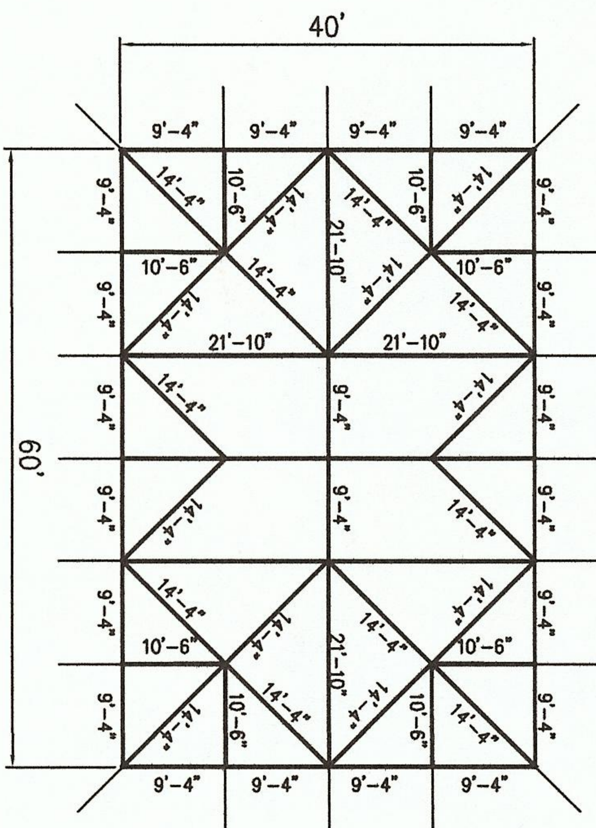
PLAN VIEW
