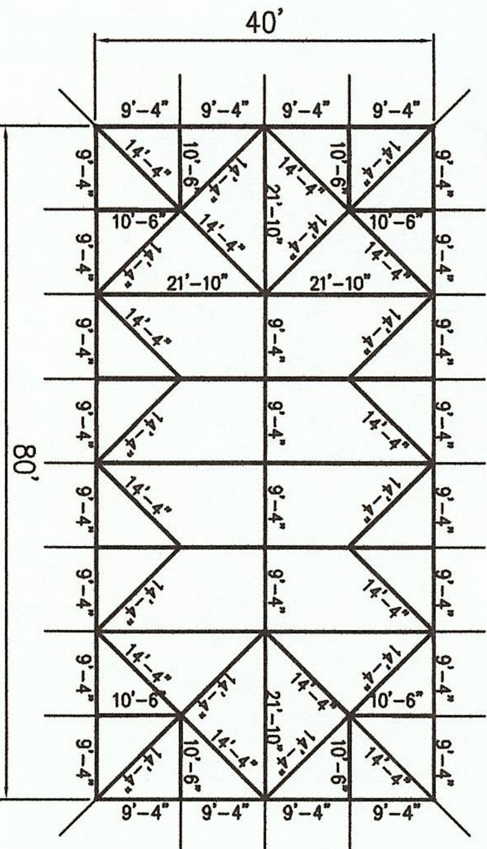
PLAN VIEW
